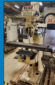
(3) Vertical Milling Machines by Bridgeport & JET up to 3 HP
